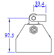
END VIEW - CONDUIT EXIT SIDE
