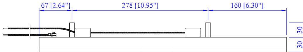
SIDE VIEW
